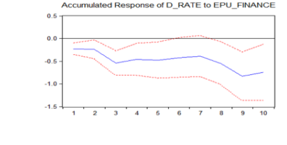
Accumulated Response to Cholesky One S.D. Innovations \pm 2 S.E.
