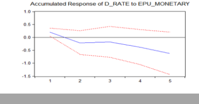
Accumulated Response to Cholesky One S.D. Innovations \pm 2 S.E.
